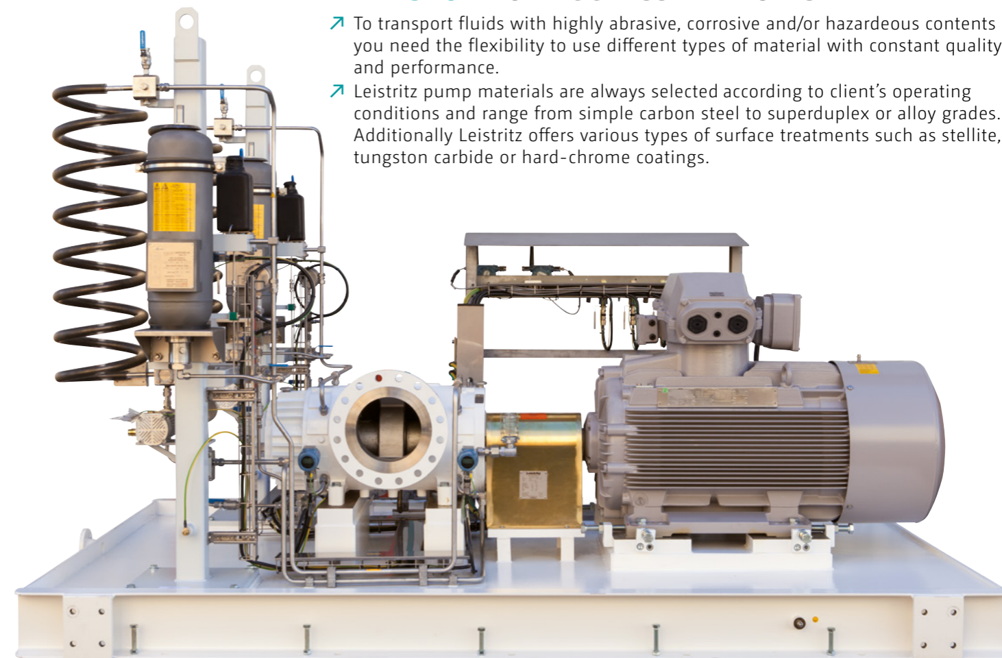
» Leistriz L4 transfer pump made of super duplex stainless steel for a client in the Middle East, specially designed and adapted to its application.«
